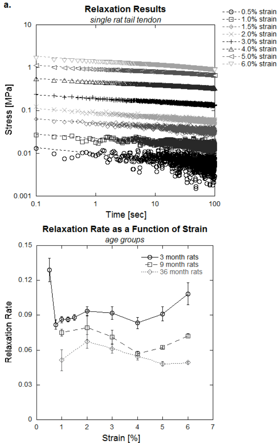
Figure 1. Relaxation as a function of strain. Relaxation data were plotted on a log-log scale and fitted with power law curves (results from a single 3 month old rat tendon without smoothing shown) (a), the slope of which is the relaxation rate (b). In paired t-tests, relaxation rates decreased significantly from 3mo to 9mo ( p = 0.0019 ) and also from 9mo to 36mo ( p = 0.0073 ) at strains of 1, 2, 3, 4, 5, and 6%. Error bars represent one standard error.
